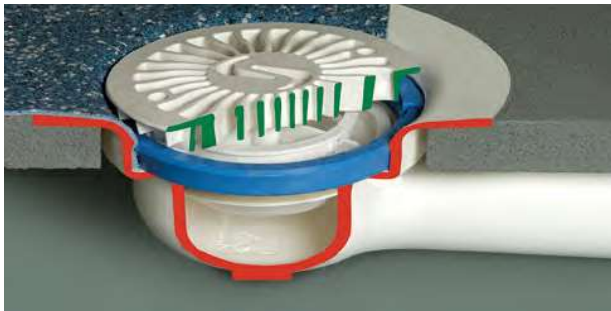
Figure 11.2 Drain with clamping ring in place
